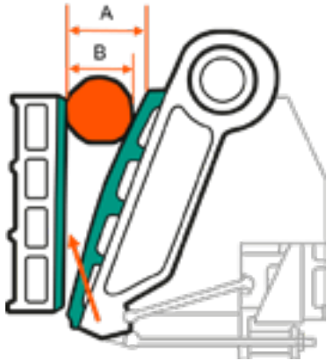
Conventional jaw crusher design:
