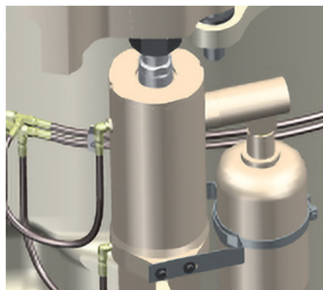
Instant recovery in case of overload thanks to accumulators connected to the tramp release cylinders
