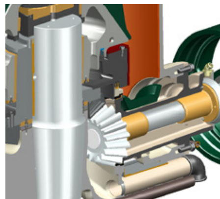
High-performance non-contact labyrinth seals
